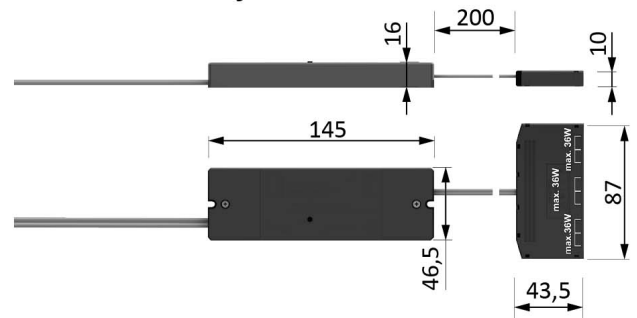
Smartempfänger des Sets 31.124.01 smart receiver of set
